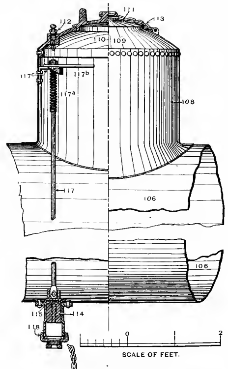
Fig. 373. Sectional Elevation of Tank, Dome and Valve.
